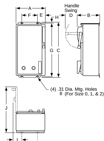
Figure 3 NEMA Type 12 Enclosure
