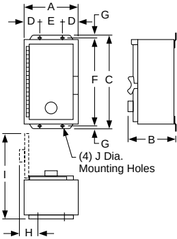
Figure 16 NEMA Type 12 Industrial Use Enclosure
