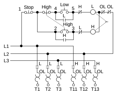
2-Speed Separate Winding Constant HP, Constant Torque and Variable Torque NEMA Size 0-4 Sizes 5, 6 & 7 Use Special Circuitry
