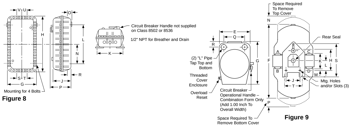
NEMA 7 & 9 SPIN TOP® Enclosure — Figure 9
