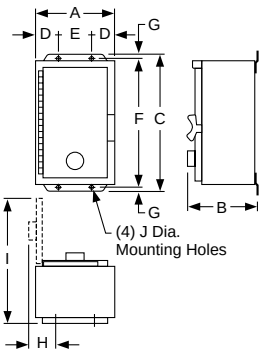
Figure 17 NEMA Type 12 Industrial Use Enclosure
