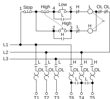
2-Speed Consequent Pole Constant Horsepower NEMA Size 0-4 Sizes 5, 6 & 7 Use Special Circuitry
