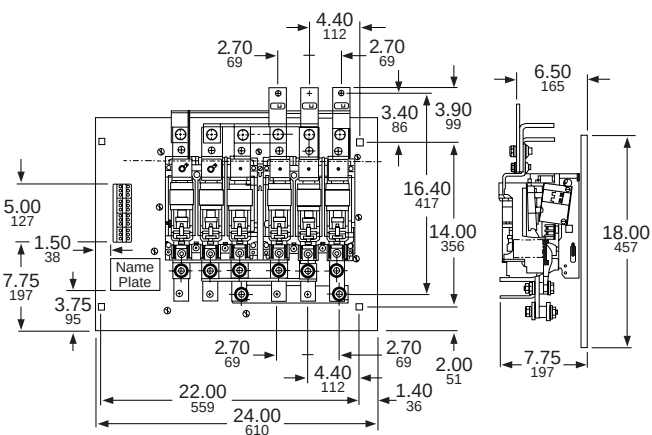
Size 6 Reversing Contactor Outline without Lugs
