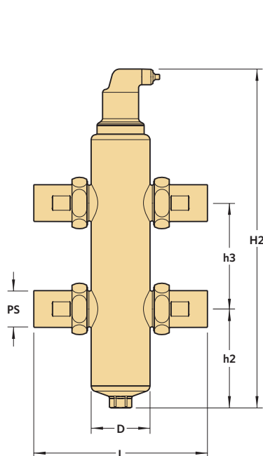
VDX Brass 1"-2" Threaded or Sweat
