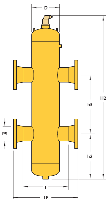
VDX Steel 2"-12" Threaded or Flanged
