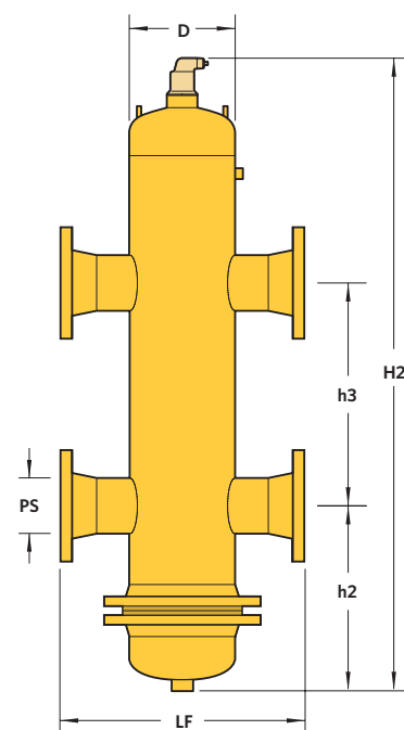
VXN Steel 2"-12" Flanged with Removable Head
