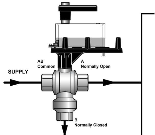
Figure 2. Three-way Diverting Application.
