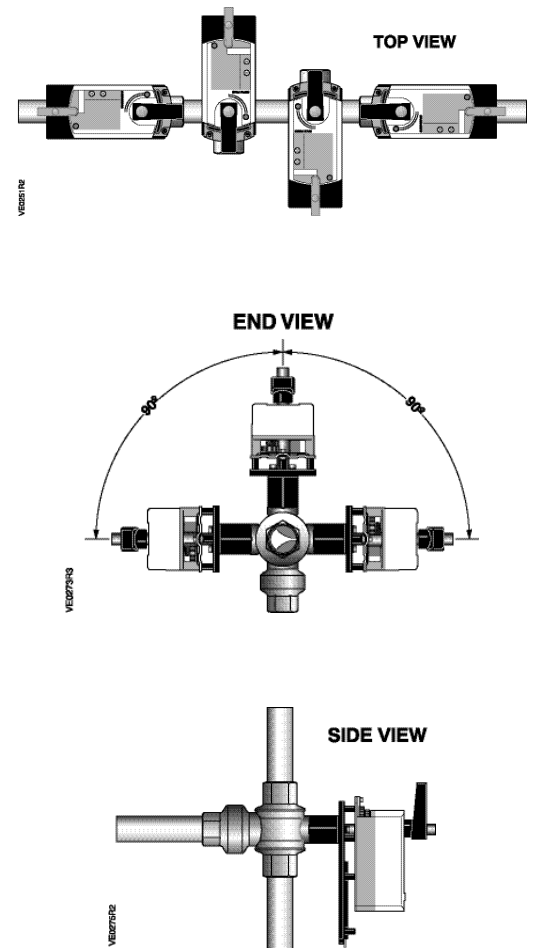
Figure 5. Mounting Positions.
