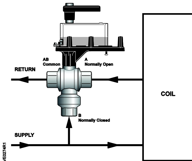
Figure 1. Mixing Application.
