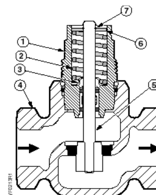
Normally Closed
