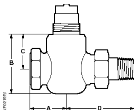
Internal Thread (IT) NPT × Union External Thread (UET) IT×UET
