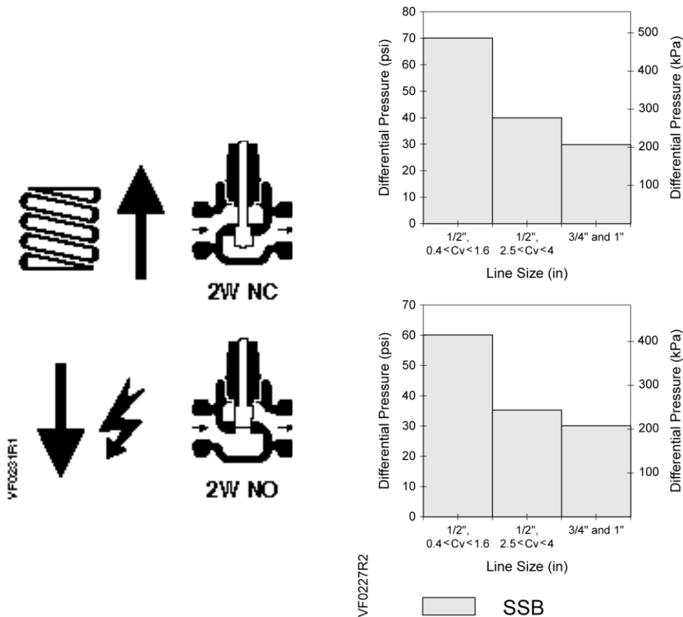
Figure 2. Close-off Pressures.
