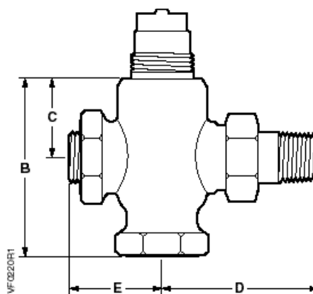
Angle Internal Thread (AIT) × Union External Thread (UET) AIT×UET
