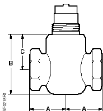
Internal Thread (IT) NPT × Internal Thread (IT) NPT IT×IT
