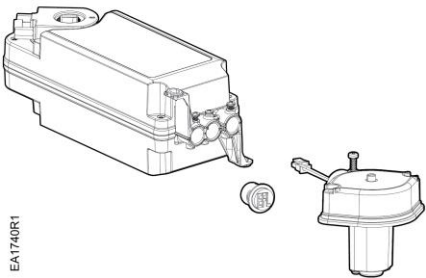
Figure 4. GVD/GKD Actuator and EFL.
