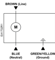
Figure 3. 230 Vac.
