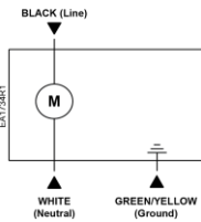
Figure 2 120 Vac.
