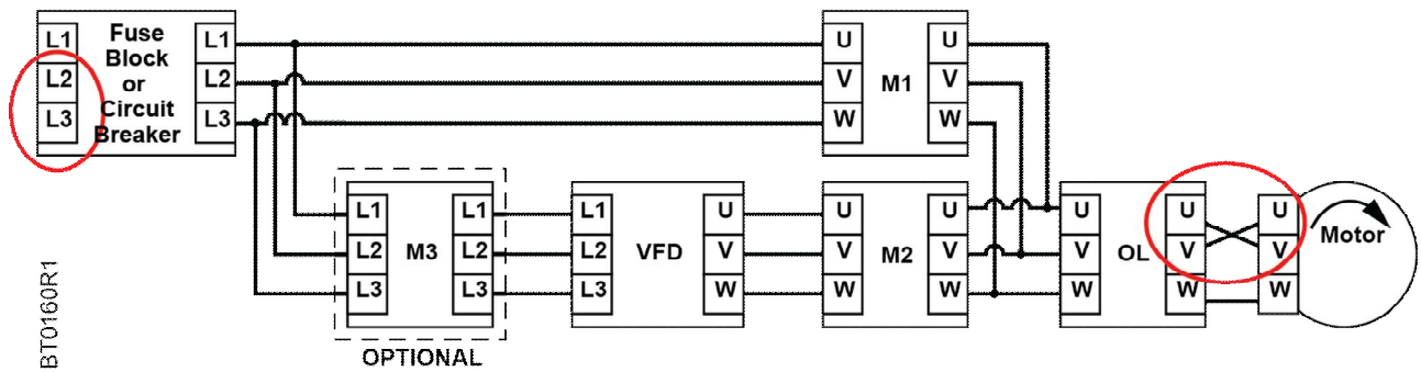
Figure 6. Rotation Correction – VFD Reversed, Bypass Correct.
