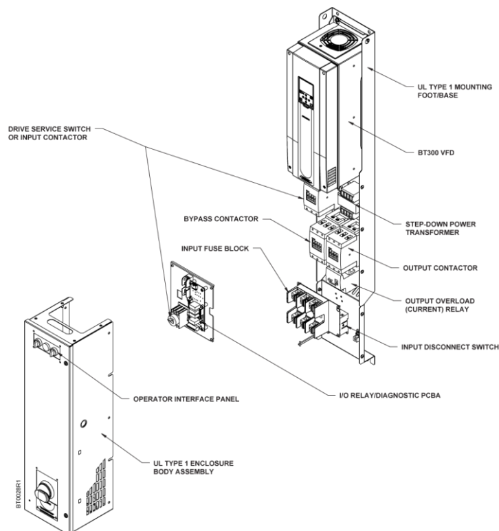
Figure 27. FS6 C-Bypass with Disconnect with Fuses Components.
