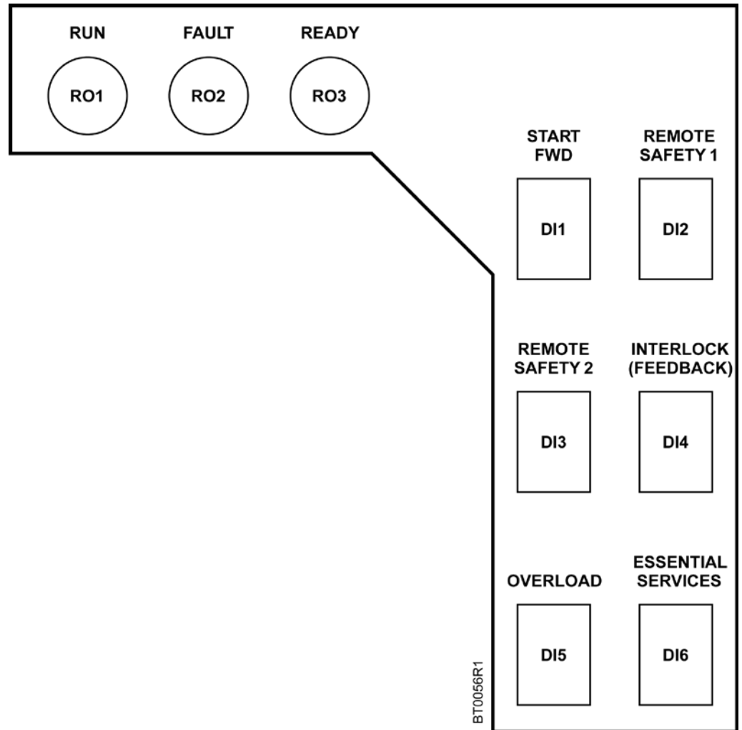
Figure 14: Bypass Overlay 1.
