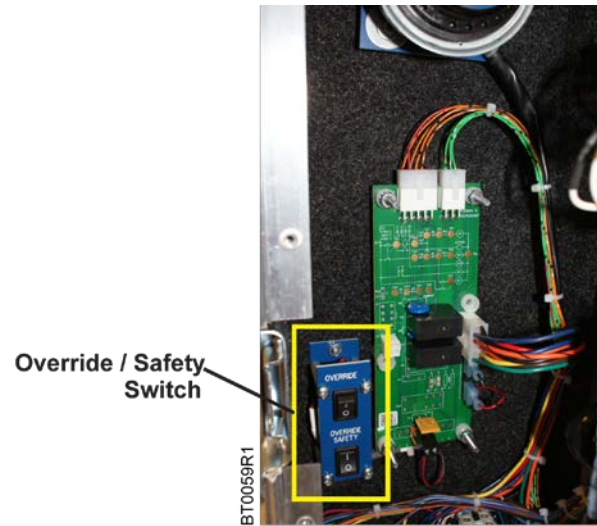
Figure 19: Override/Safety Switches.
