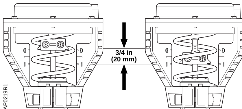
Figure 1. Actuator Operation.
