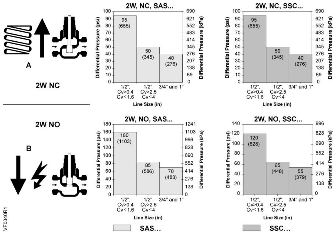
Figure 2. Close-off Pressures.
