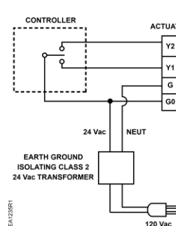
Figure 7. For Non-Triac Driven Controllers.
