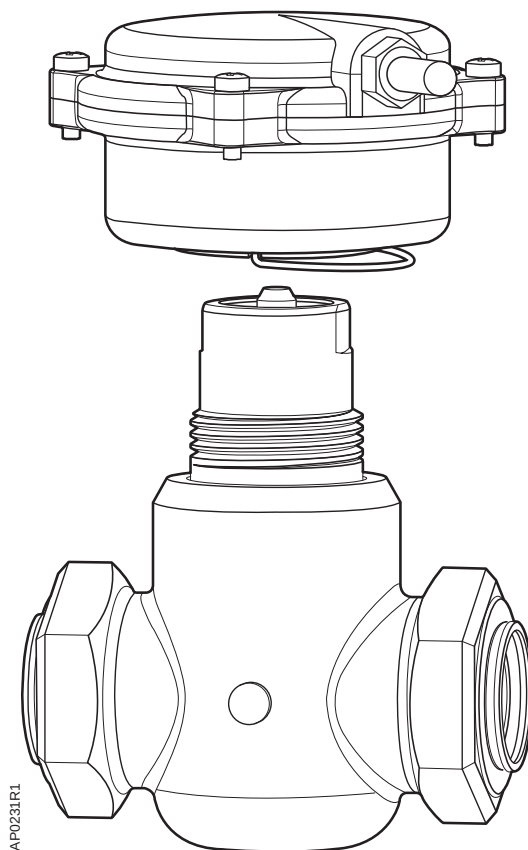
Figure 2. Two-inch Actuator and Powermite Valve.
