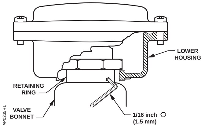
Figure 1. Securing the Retaining Ring before Removing the Actuator from a Valve.
