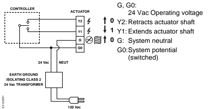
Figure 9. SSD81.5U Floating Control SR Hot-Switch.
