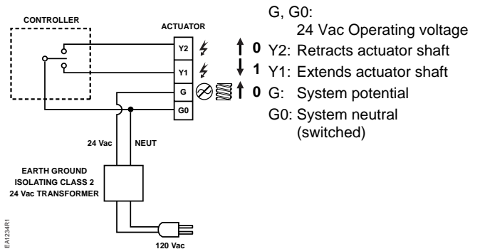
Figure 10. SSD81.5U Floating Control SR Neutral Switching Applications.
