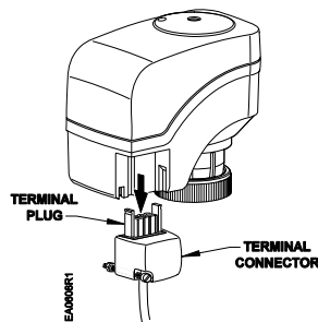
Figure 15. Removing Terminal Plug.
