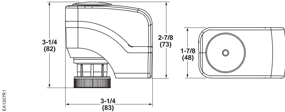
Figure 17. SSD61U/SSD81U Actuator in Inches (Millimeters).
