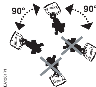
Figure 2. Acceptable Mounting Position with Valve.
