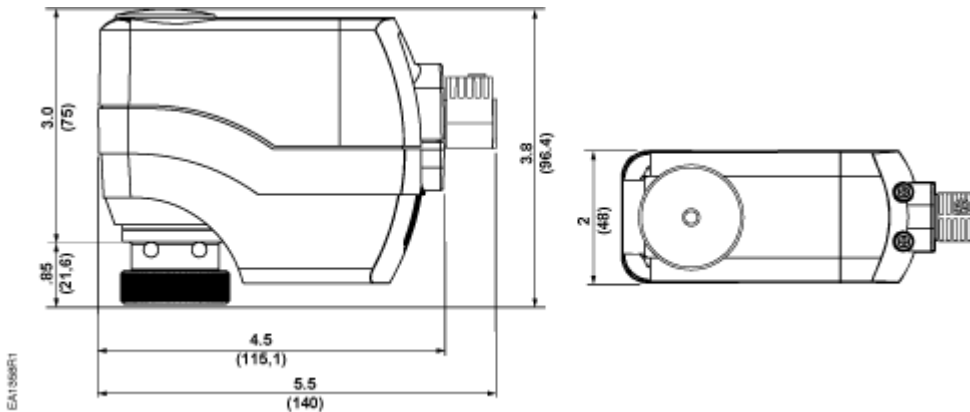
Figure 18. SSD61.5U/SSD81.5U Actuator Dimensions in Inches (Millimeters).
