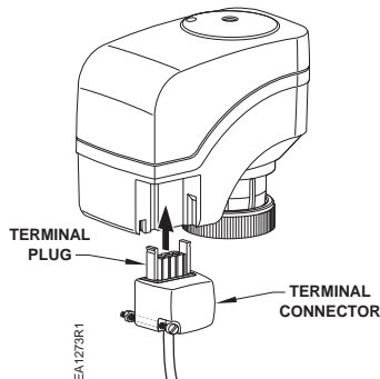
Figure 5. Insert Terminal Connector.
