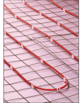
Uniform layout ensures even radiant heating surface.
