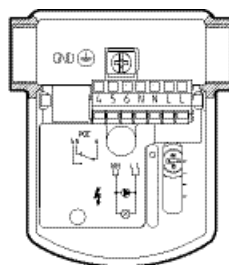
SKP55.011U..
