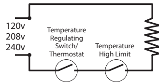
Non-switched Wiring Diagram
