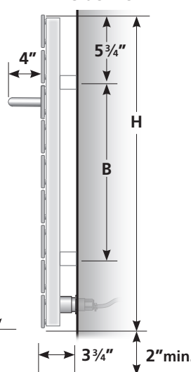
9 Panel Omnipanel II Side View
