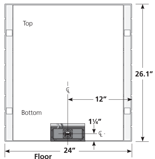
9 Panel Omnipanel II Back View
