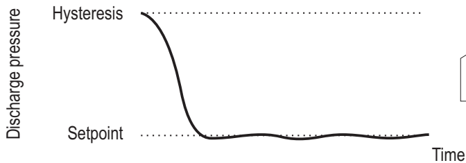
Proportional + Integral Control
