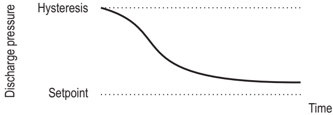
Proportional-only control
