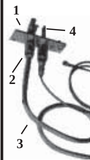
FIGURE 9 - Vertical Spark Pilot for Models RPV, RPBE, RPVE, RPVJ, RPAK, HRPV, HRPBE, HRPVE, CRPV, HCRPV, CRPBE, HCRPBE, CRPVE, HCRPVE; CRPVAK prior to Series 6 and RCG 7-12/, 10 ton equipped with G60 or G67 ignition Controller
