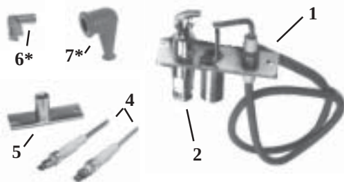
FIGURE 9 - Vertical Spark Pilot for Models RPV, RPBE, RPVE, RPVJ, RPAK, HRPV, HRPBE, HRPVE, CRPV, HCRPV, CRPBE, HCRPBE, CRPVE, HCRPVE; CRPVAK prior to Series 6 and RCG 7-12/, 10 ton equipped with G60 or G67 ignition Controller
