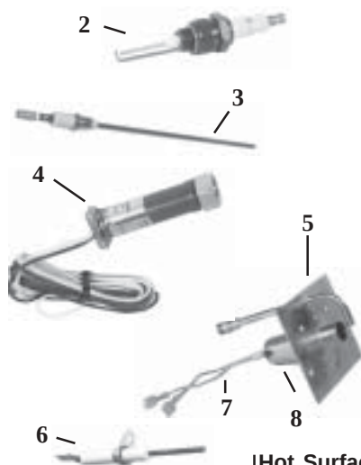
FIGURE 11 - Pilot Systems used on Direct-Fired Models RDF/ADF/ADFH/DFA/DV
