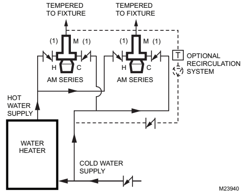
Fig. 3. AM Series ASSE 1070 - Handleless Fixtures
