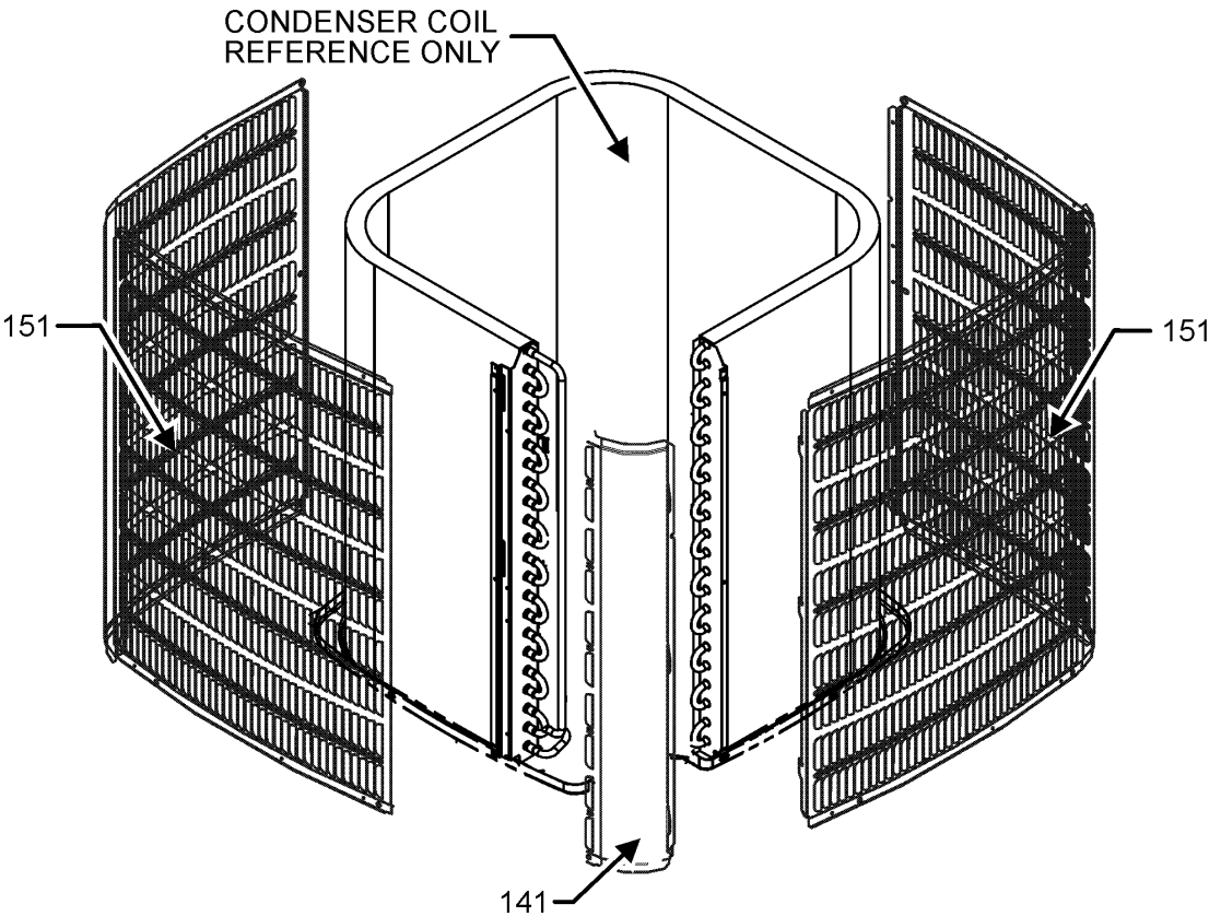
LOUVER PANEL ASSEMBLY
