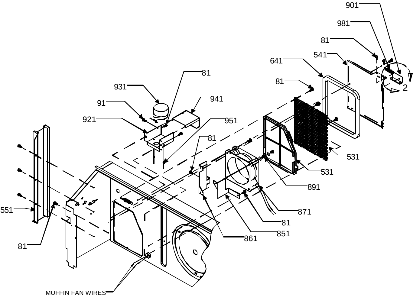
MODELS WITH POWERVERT OR POWER DOOR
