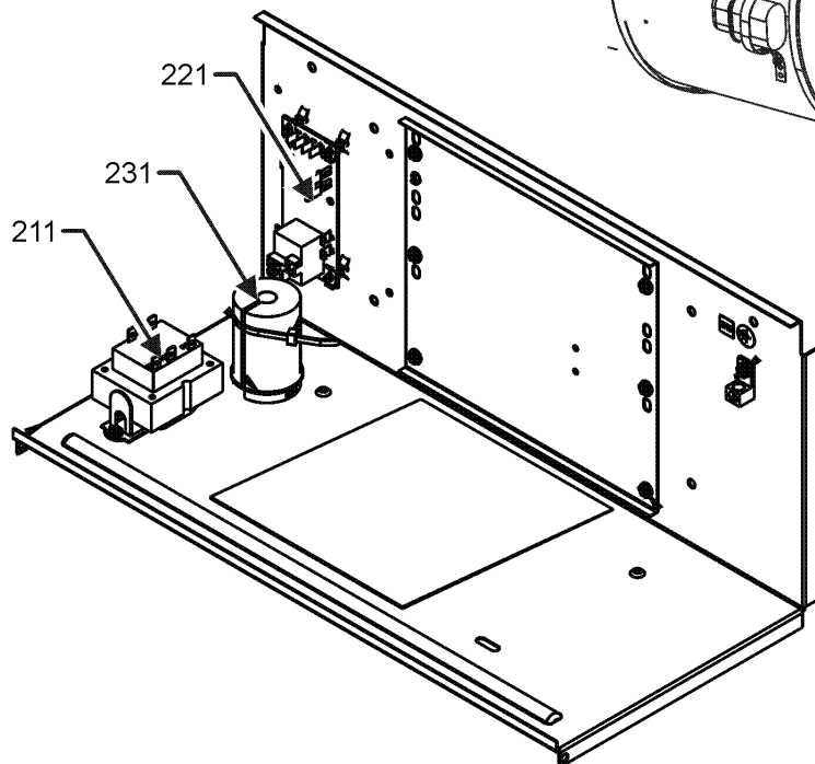
CONTROL PANEL ASSEMBLY
