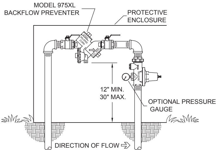
OUTDOOR INSTALLATION
