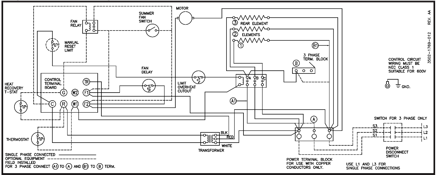
Diagram 11: 3 Element, Single and Three Phase
