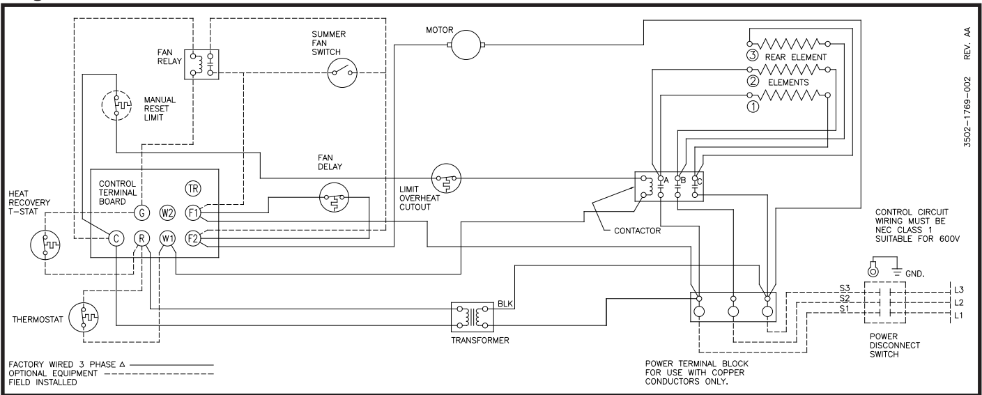
Diagram 2: 3 Element, Three Phase
