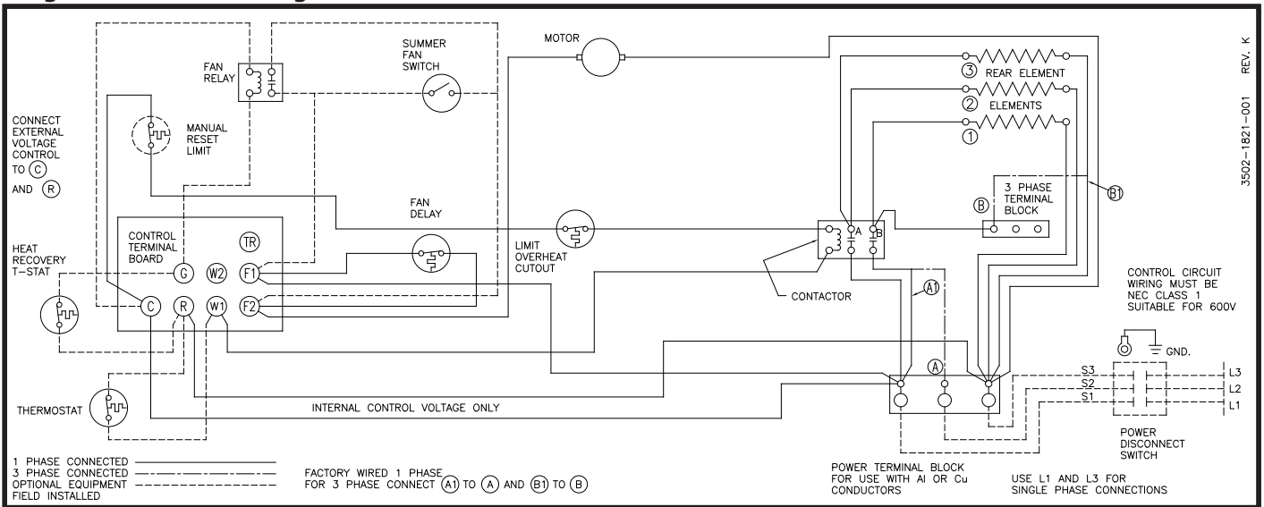
Diagram 4: 3 Element, Single and Three Phase
