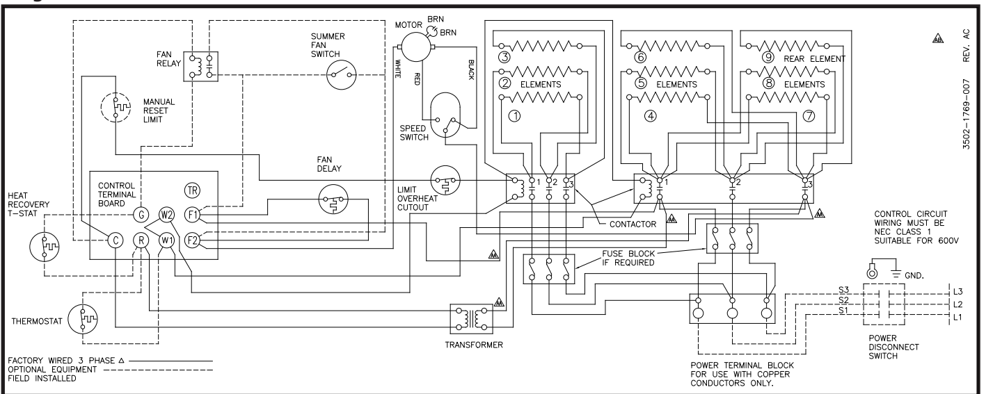
Diagram 8: 9 Element, 2 Contactor, Three Phase
