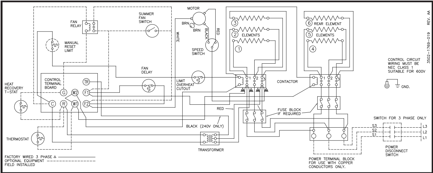
Diagram 13: 6 Element, 2 Contactor, Three Phase
