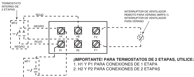
Figura 4. Bornera de control (para calefactores sin contactor)
