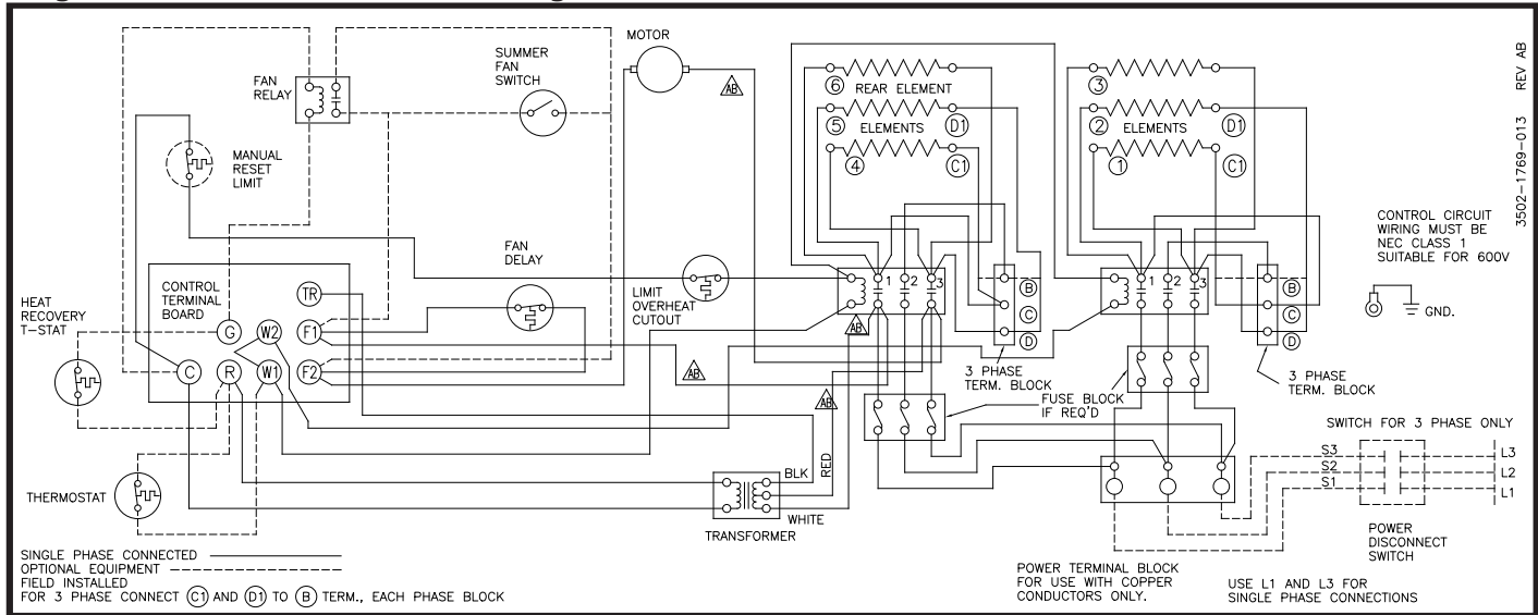
Diagram 10: 6 Element, 2 Contactor, Single and Three Phase
