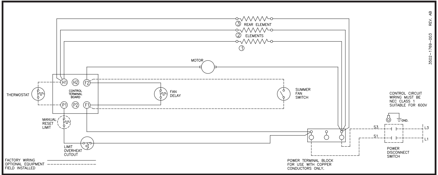
Diagram 3: 3 Element, Single Phase
