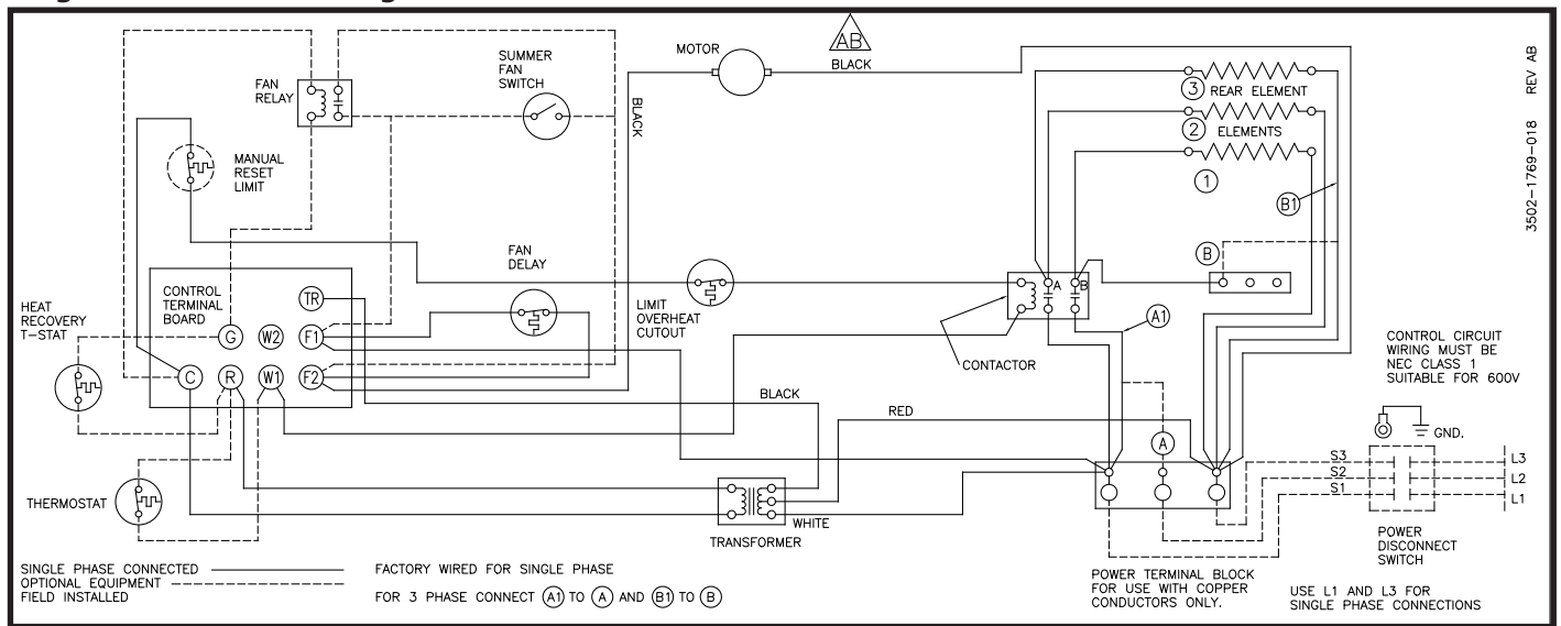
Diagram 12: 3 Element, Single and Three Phase
