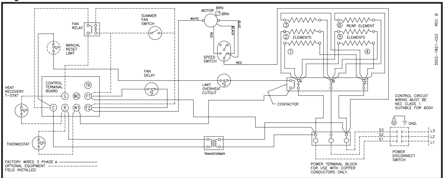
Diagram 6: 6 Element, Three Phase
