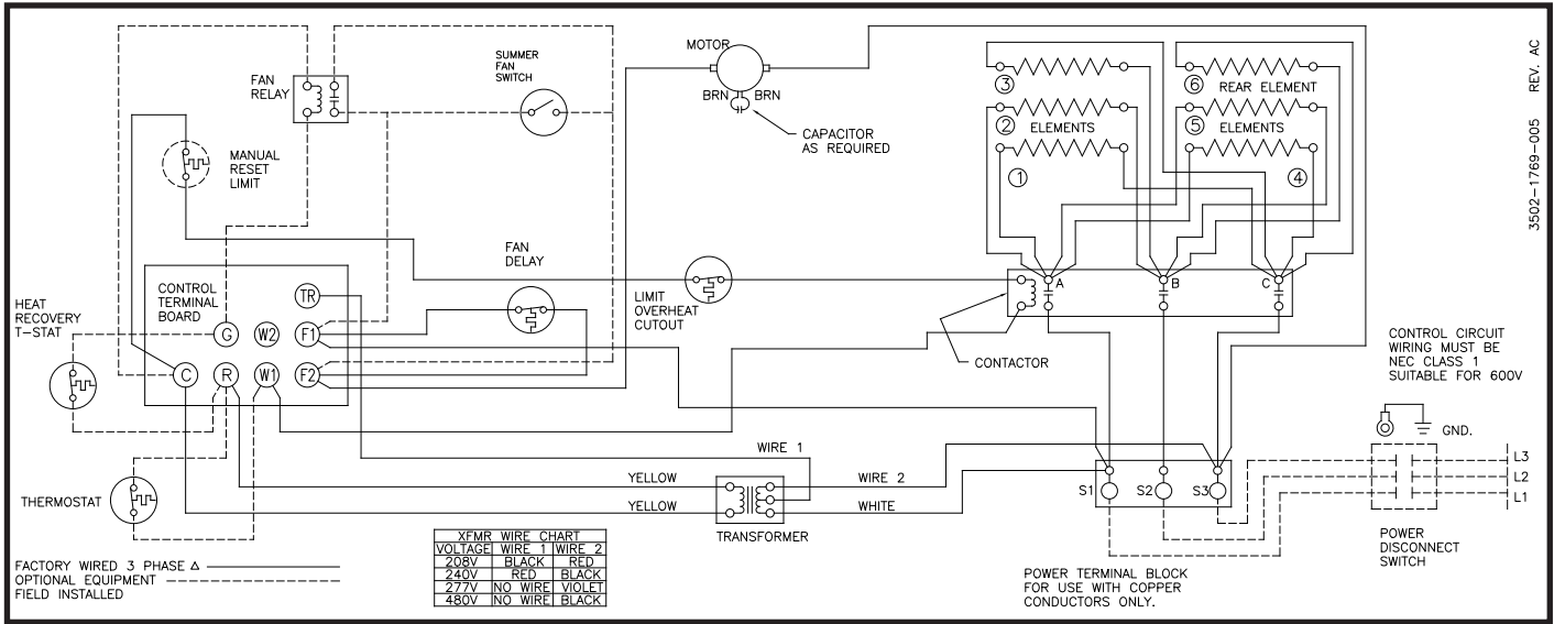
Diagram 5: 6 Element, Three Phase
