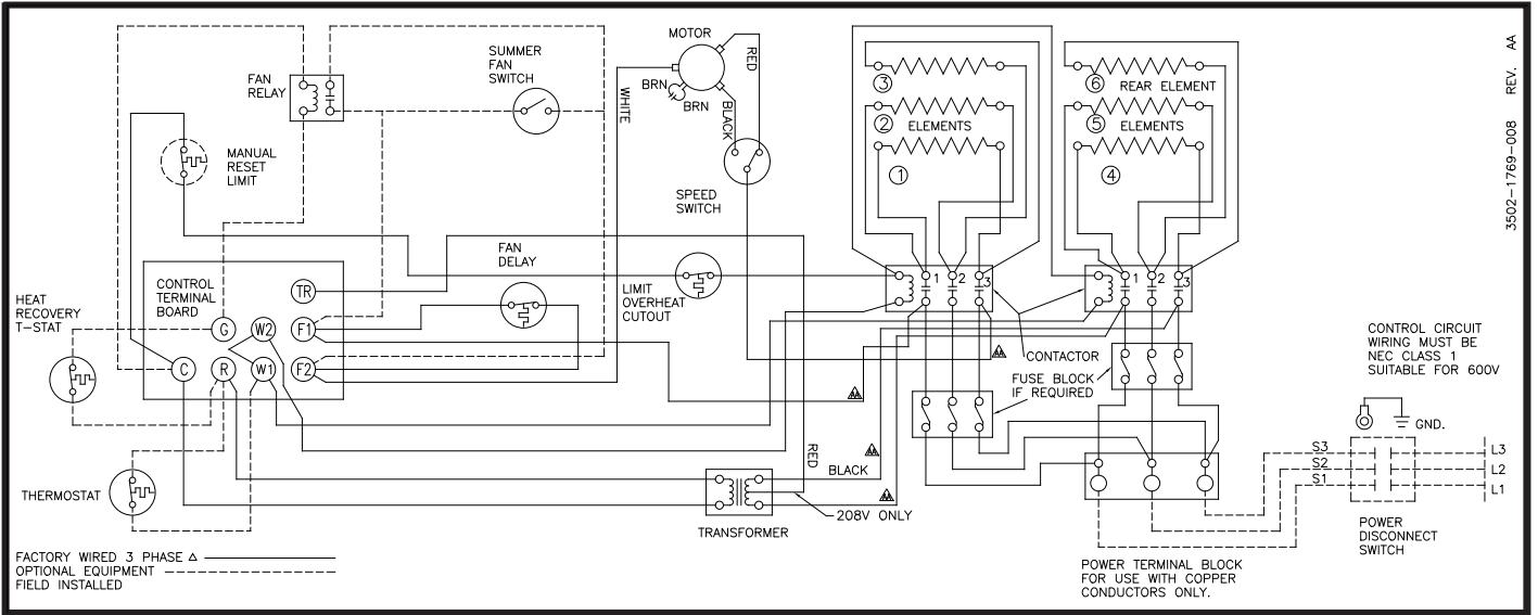
Diagram 7: 6 Element, 2 Contactor, Three Phase
