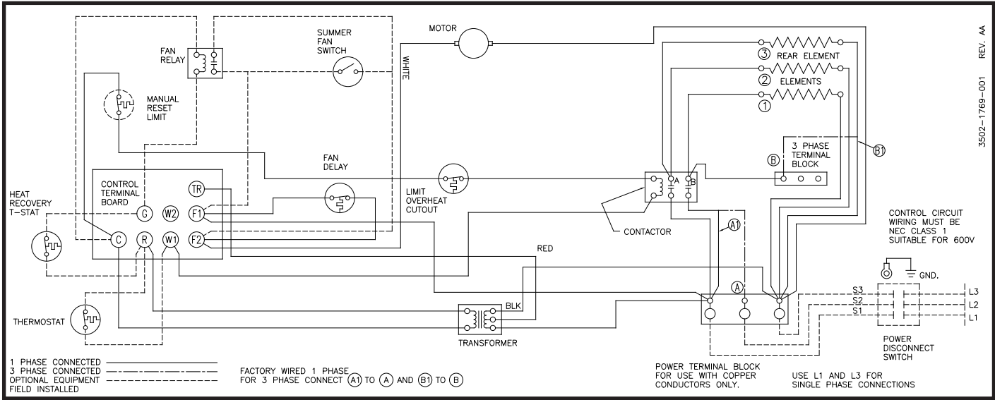
Diagram 1: 3 Element, Single and Three Phase
