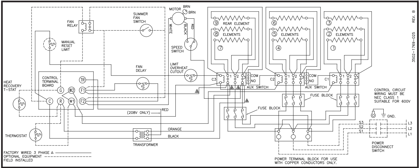
Diagram 9: 9 Element, 3 Contactor, Three Phase
