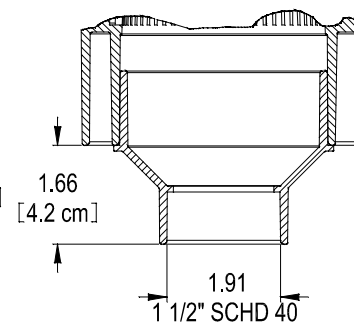
OPTIONAL 1 1/2" REDUCER PART NO. PCF-PLVF-15
