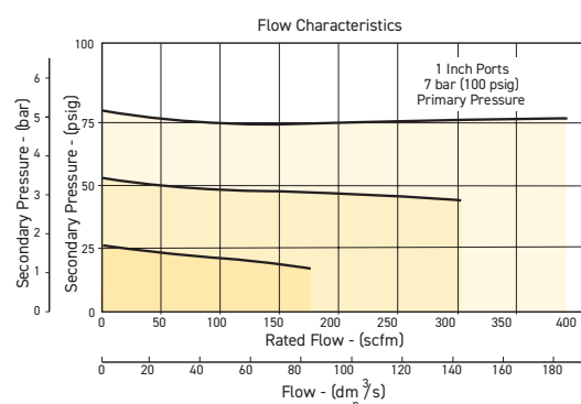
R119 1" Regulator
