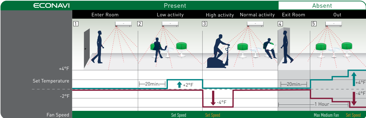
Legend: - - - Set Temperature — Cooling Power — Heating Power Remark: Set temperature on remote control display remains unchanged.
