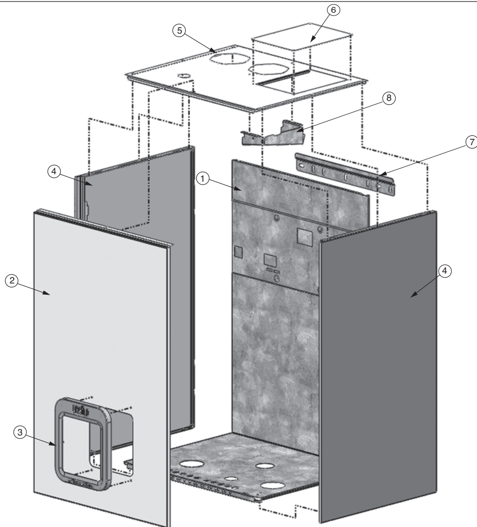
Fig.35: PRESTIGE Solo 399 Jacket Components
