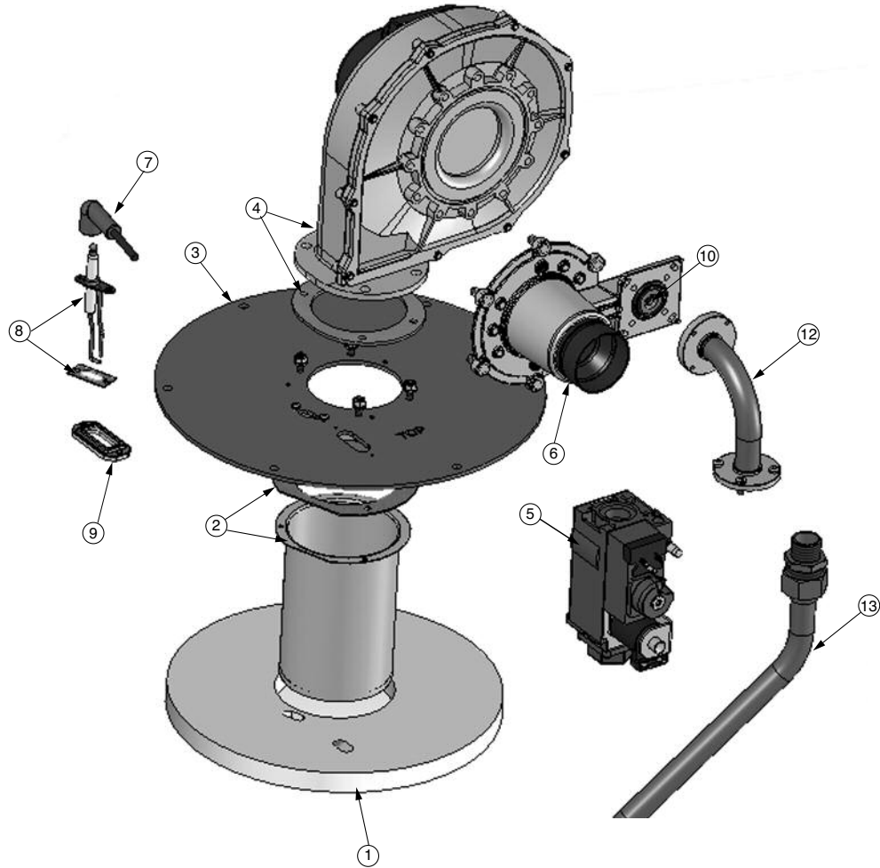
Fig. 28A: PRESTIGE Solo 399 Burner Components
