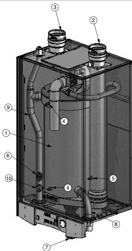
Fig. 27A: PRESTIGE Solo 175/250 Internal Components
