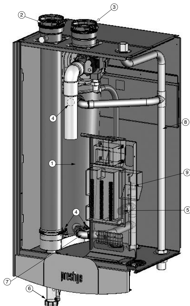
Fig. 27: PRESTIGE Solo 60 Internal Components
