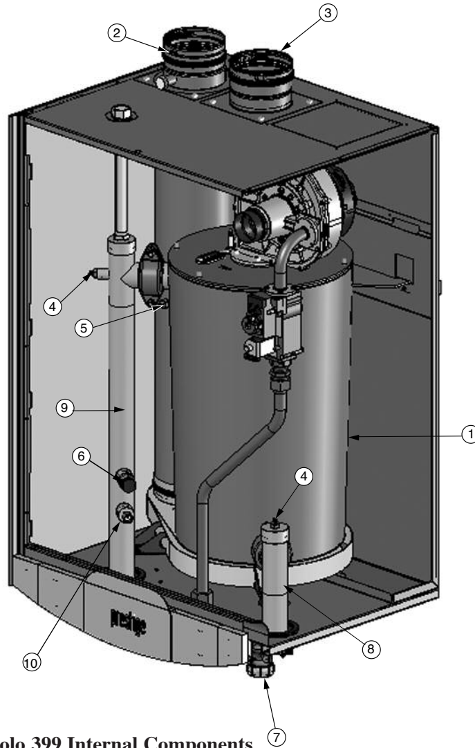
Fig. 27B: PRESTIGE Solo 399 Internal Components
