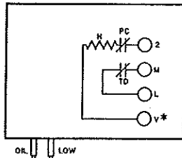
P45AAA, P45NAA
