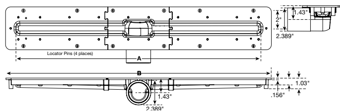
DIMENSIONS (2" SIDE WASTE OUTLET)
