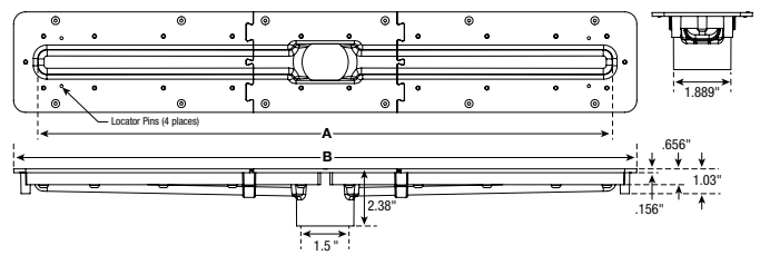
DIMENSIONS (1-1/2" VERTICAL WASTE OUTLET)
