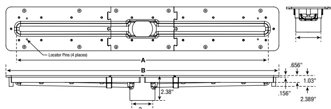
DIMENSIONS (2" VERTICAL WASTE OUTLET)
