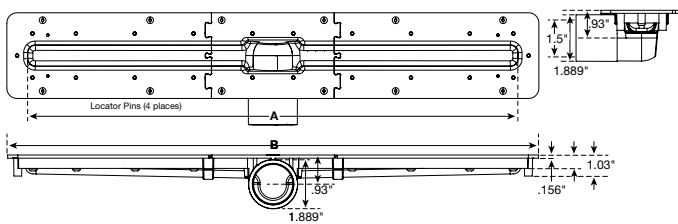
DIMENSIONS (1-1/2" SIDE WASTE OUTLET)
