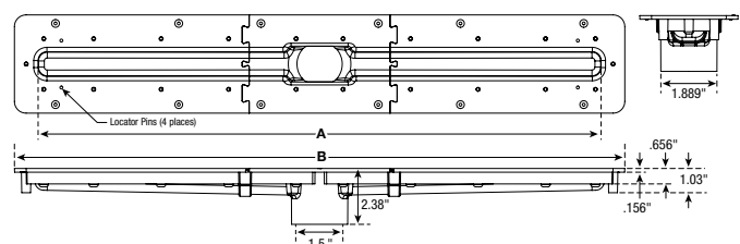
DIMENSIONS (1-1/2" VERTICAL WASTE OUTLET)
