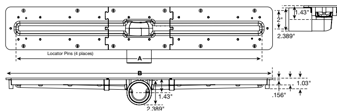
DIMENSIONS (2" SIDE WASTE OUTLET)
