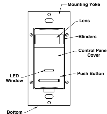
Figure 2: Sensor Features
