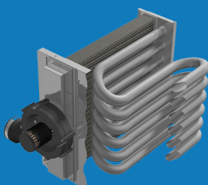
MODINE CONSERVICORE® HEAT EXCHANGER
