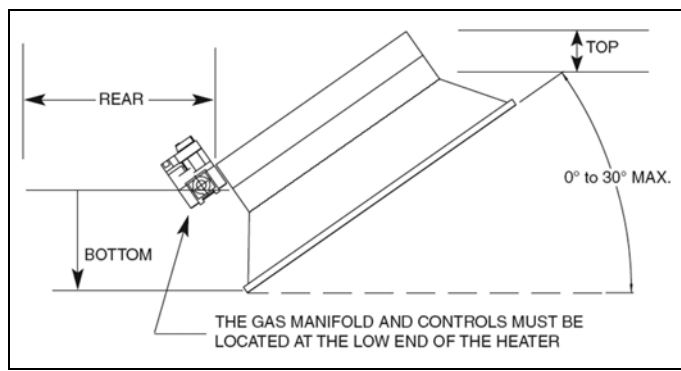
Figure 5.1 – High Intensity Clearance to Combustibles
