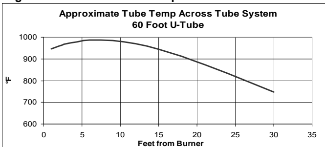
Figure 4.2 – 60 Ft U-Tube Temperature Distribution ①
