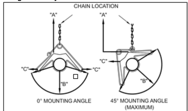
Figure 5.3 – Low Intensity Clearance to Combustibles Straight Tube Systems
