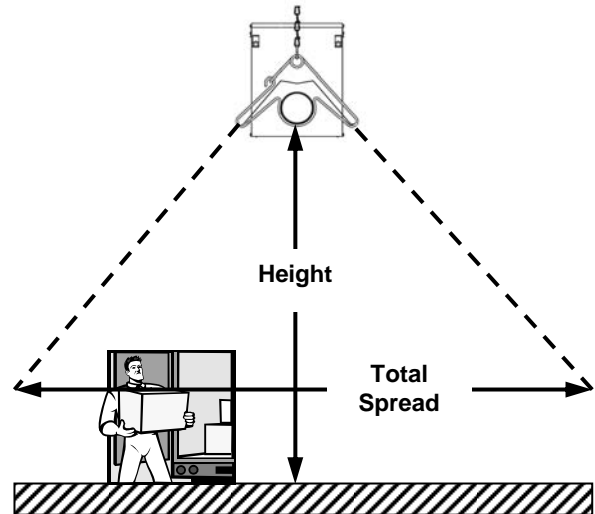
Figure 3.3 – Low Intensity Heat Spread Width
