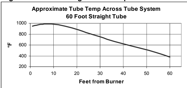
Figure 4.1 – 60 Ft Straight Tube Temperature
