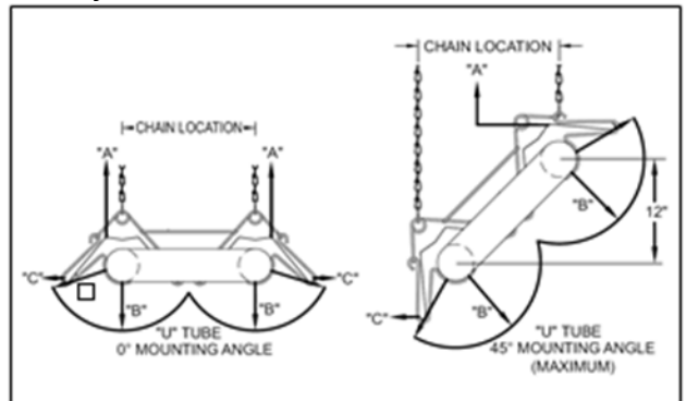
Figure 5.4 – Low Intensity Clearance to Combustibles U-Tube Systems and U-Tube
