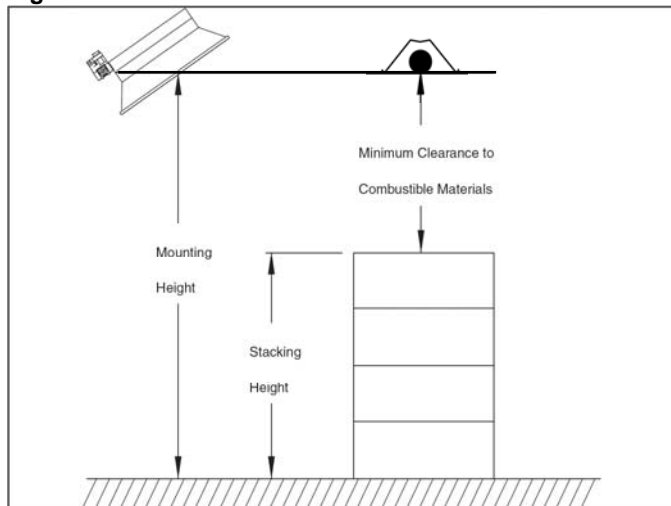
Figure 5.2 – Clearance to Stored/Stacked Materials
