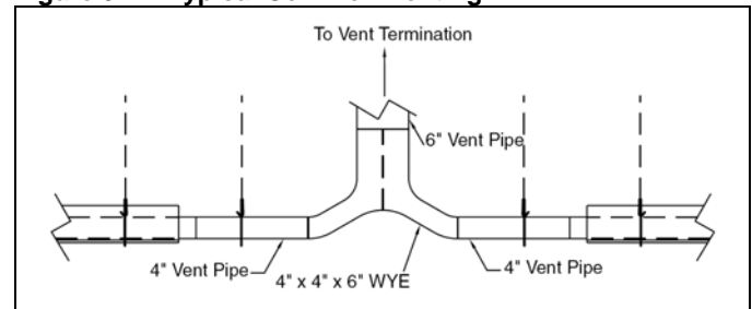
Figure 9.2 – Typical Common Venting
