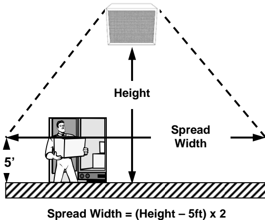
Figure 3.1 – High Intensity Heat Spread Width
