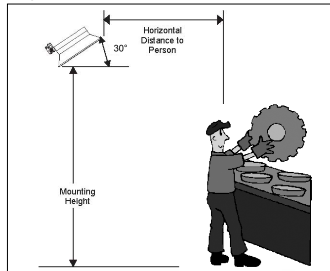
Figure 6.1 – Typical Spot Heater Mounting (Single Heater Shown)
