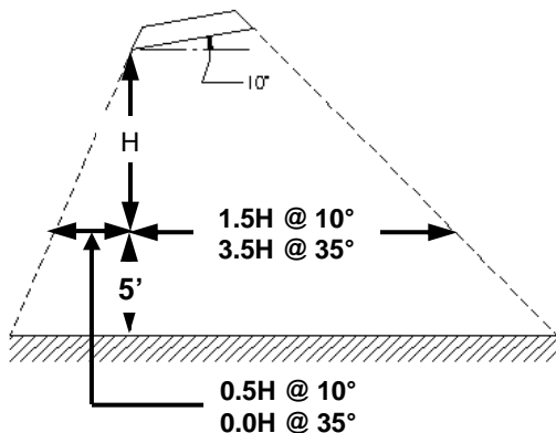
Figure 3.2 – High Intensity Heat Distribution/Throw
