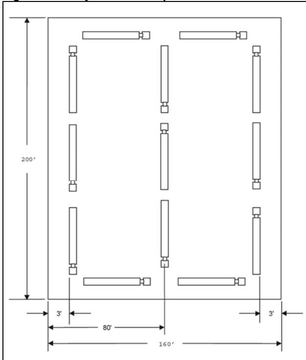
Figure 9.1 – Layout for Example 2
