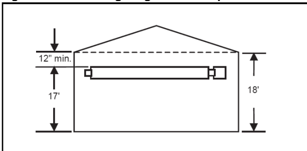
Figure 8.1 - Mounting Height for Example 1
