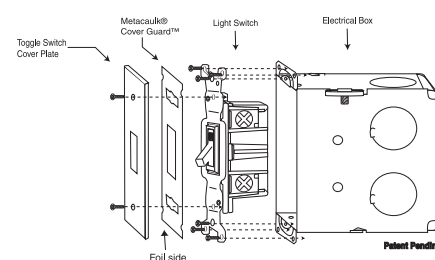
Installation of Single Electrical Switch
