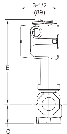
Figure-9 Mx51-710x with 3-Way Globe Valve.
