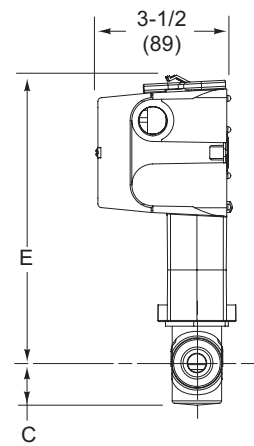
Figure-9 Mx51-710x with 3-Way Globe Valve.
