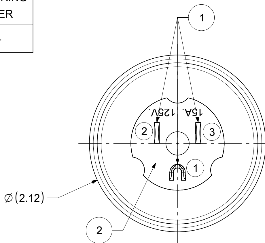
NEMA 5-15 PLUG 15A/125V
