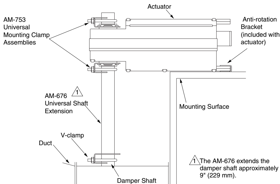
Figure-8 Installation of Universal Shaft Extension.
