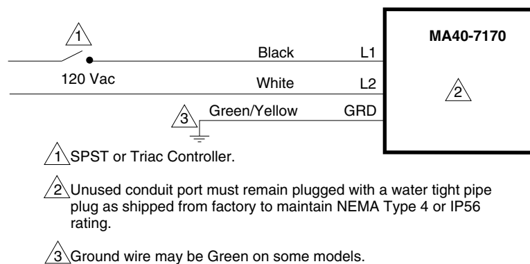
Figure-1 Typical MA40-7170 Wiring Diagram.
