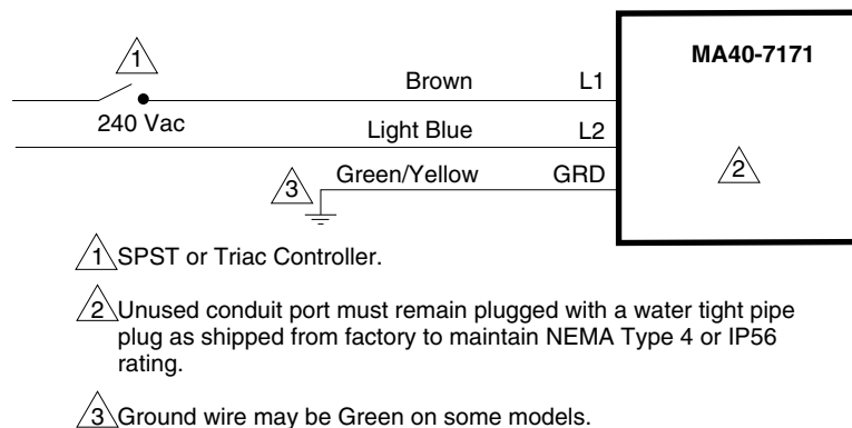
Figure-2 Typical MA40-7171 Wiring Diagram.
