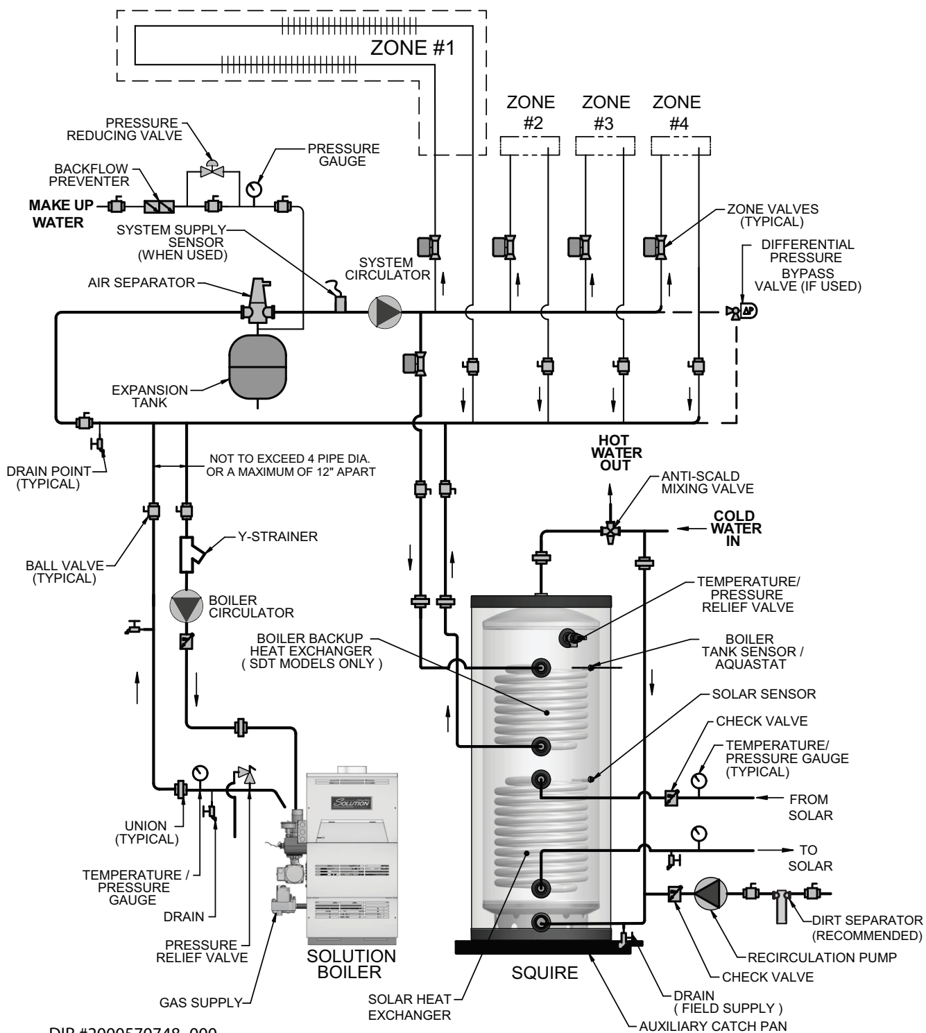
Figure 3-2 Piping Diagram Zoned with Valves
