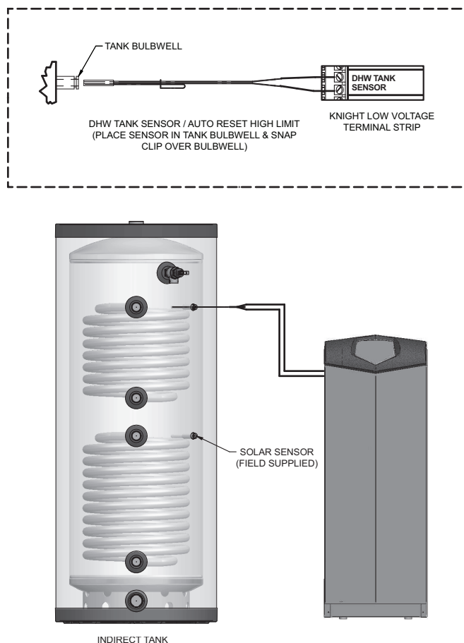
Figure 5-3 Indirect Water Heater Controlled Using Tank Sensor
