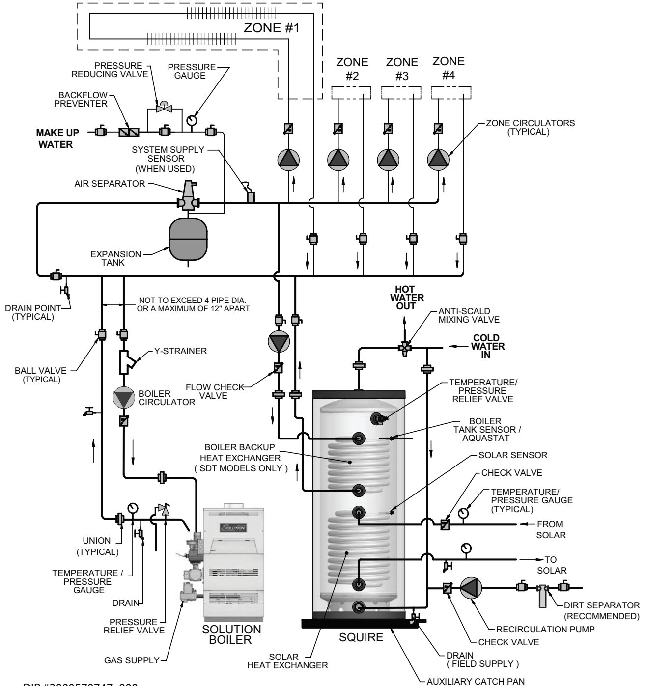
Figure 3-1 Piping Diagram Zoned with Circulators
