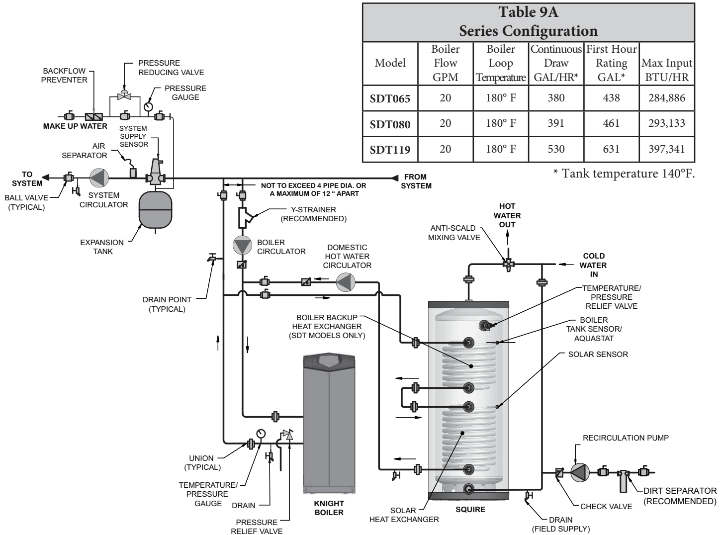
Figure 9-1 Indirect Boiler with Series Piping
