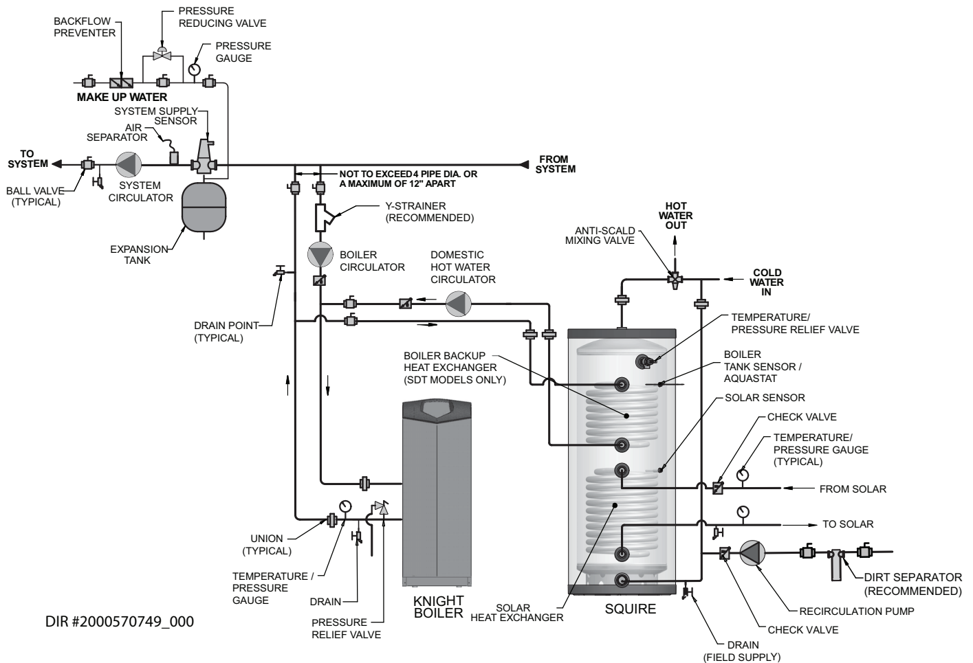
Figure 3-3 Knight Boiler Primary / Secondary Piping
