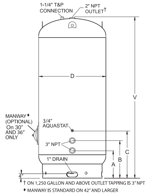
30" DIAMETER AND LARGER TANKS
