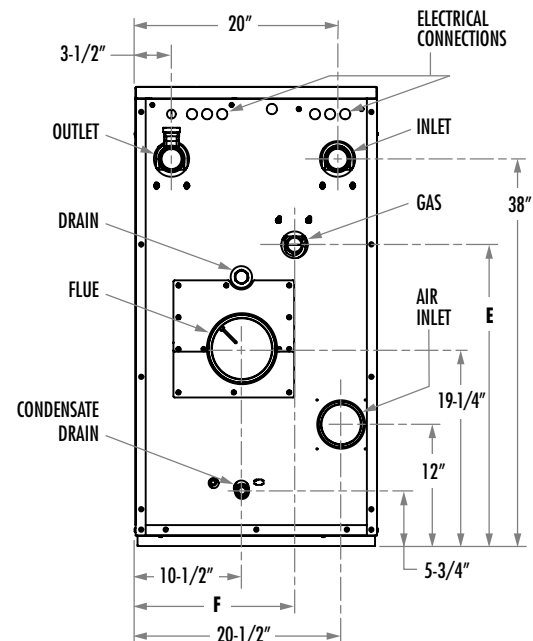
BACK VIEW
