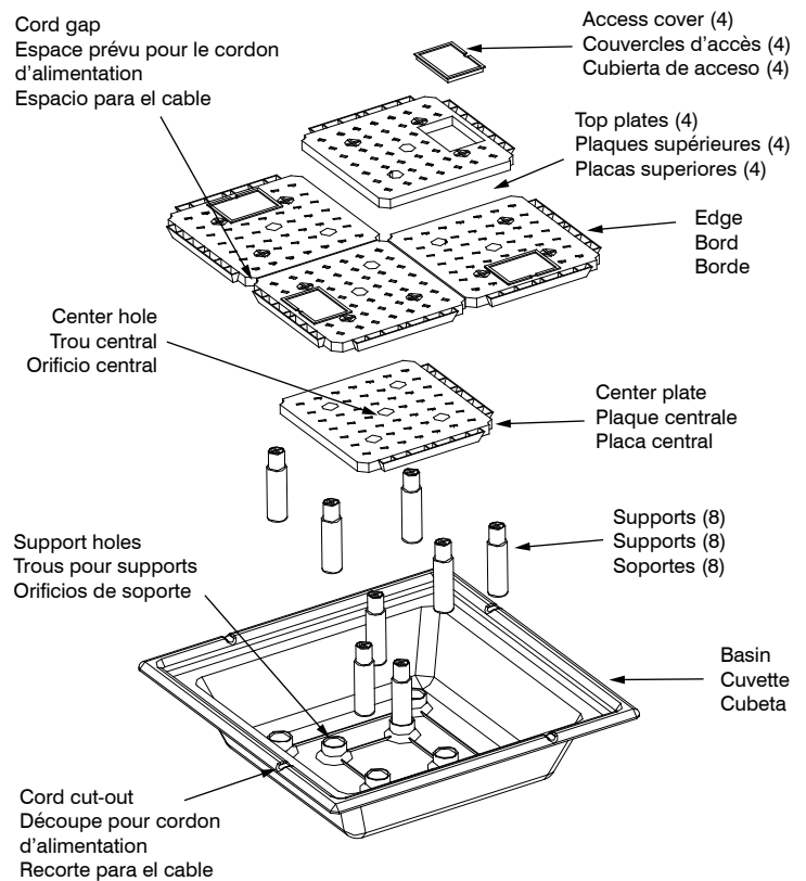
Fig. 3 - DFB44
