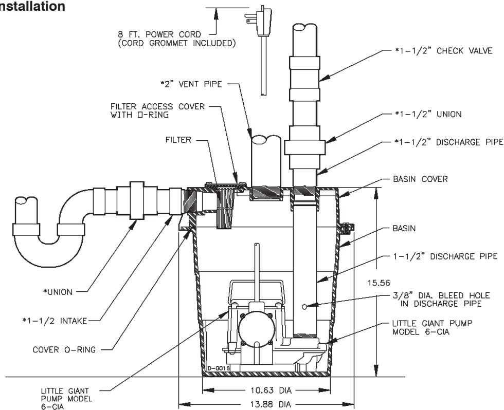
Figure 1 - Typical Installation
