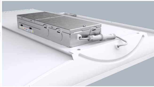
Driver box sits on top of fixture
