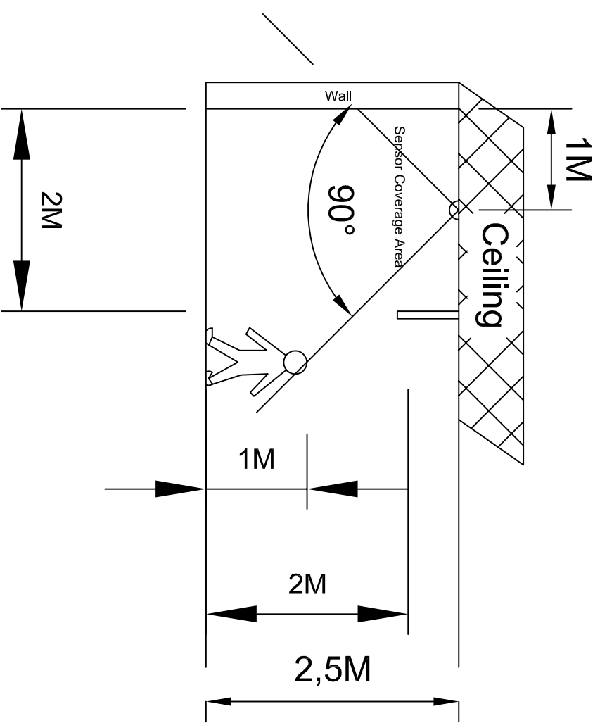
Ceiling Mount
