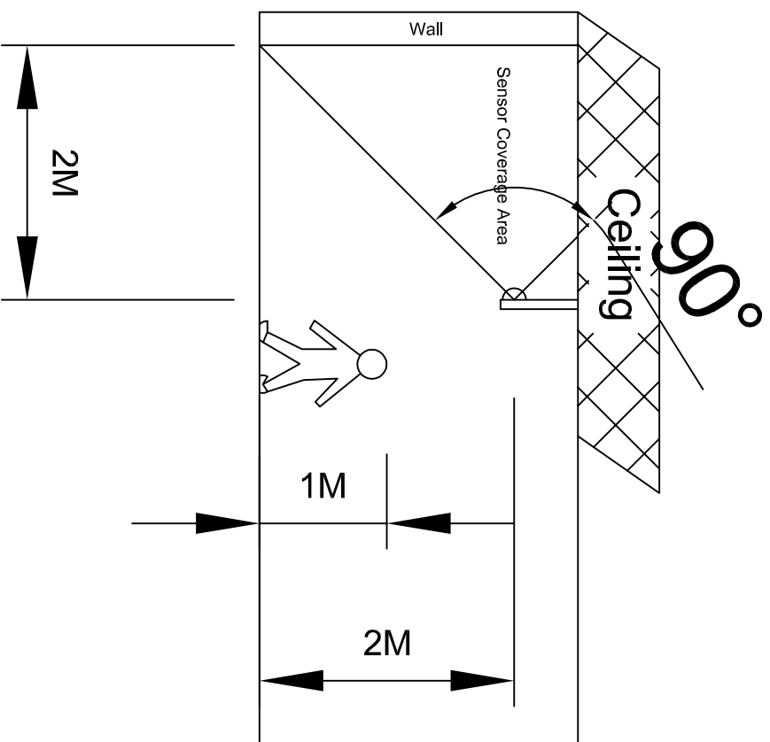
Wall Mount
