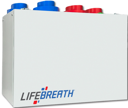
180 ERVD-FID 178 CFM @ 0.3 (75) IN. W.G. (PA)
